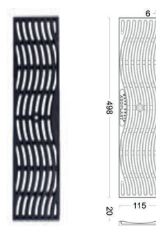
Ductile Iron Grating
