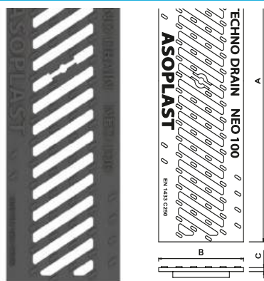
Ductile iron grating (10mm slot)
